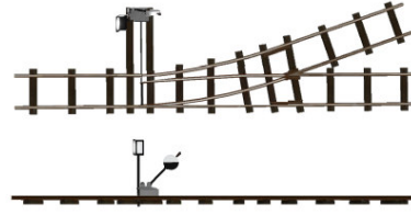
600mm_EW_19110Hr_GA_KK1 600mm EW 19° R10 Hebel l GA (S12 Holz)
